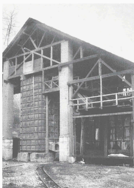
Fig. 3. Shaft furnace (Exeli system, 1872).
