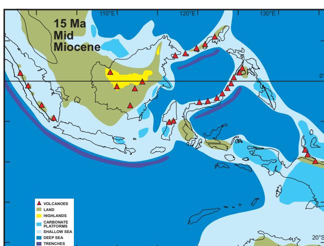
Fig. 12 Postulated distribution of land and sea in the Wallacea region at 15 Ma.
