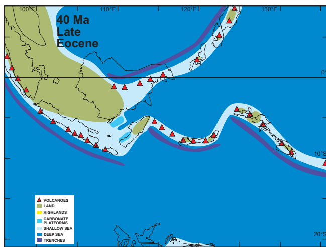
Fig. 8 Postulated distribution of land and sea in the Wallacea region at 40 Ma.
